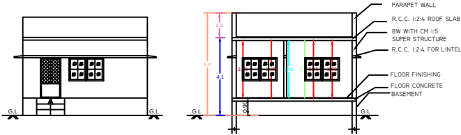
FRONT ELEVATION
