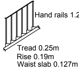
STAIR DETAILS
