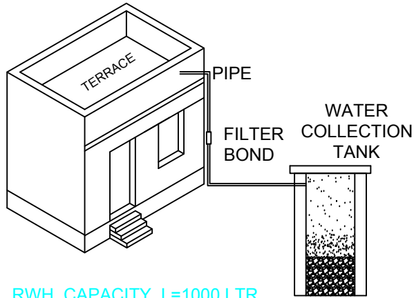
RAIN WATER HARVEST
