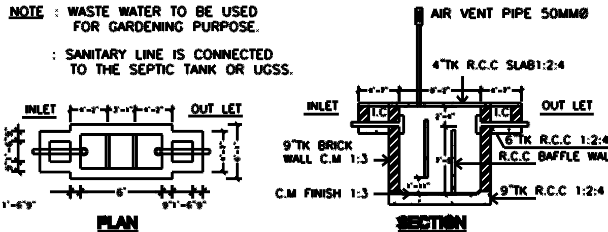
SEPTIC TANK DETAILS
