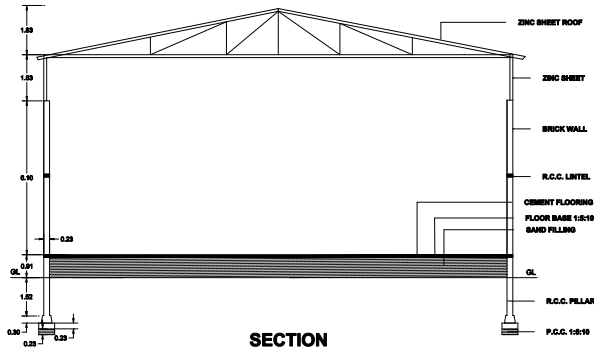
SECTION
