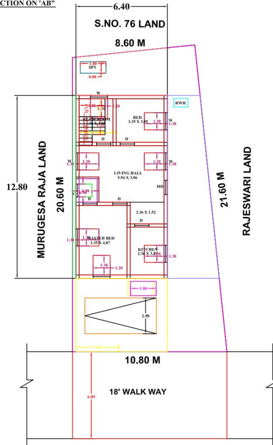
SITE & GROUND FLOOR PLAN
