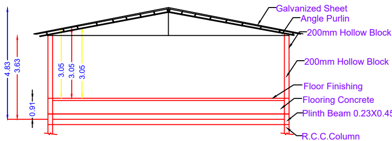
SECTION ON "PQ"
