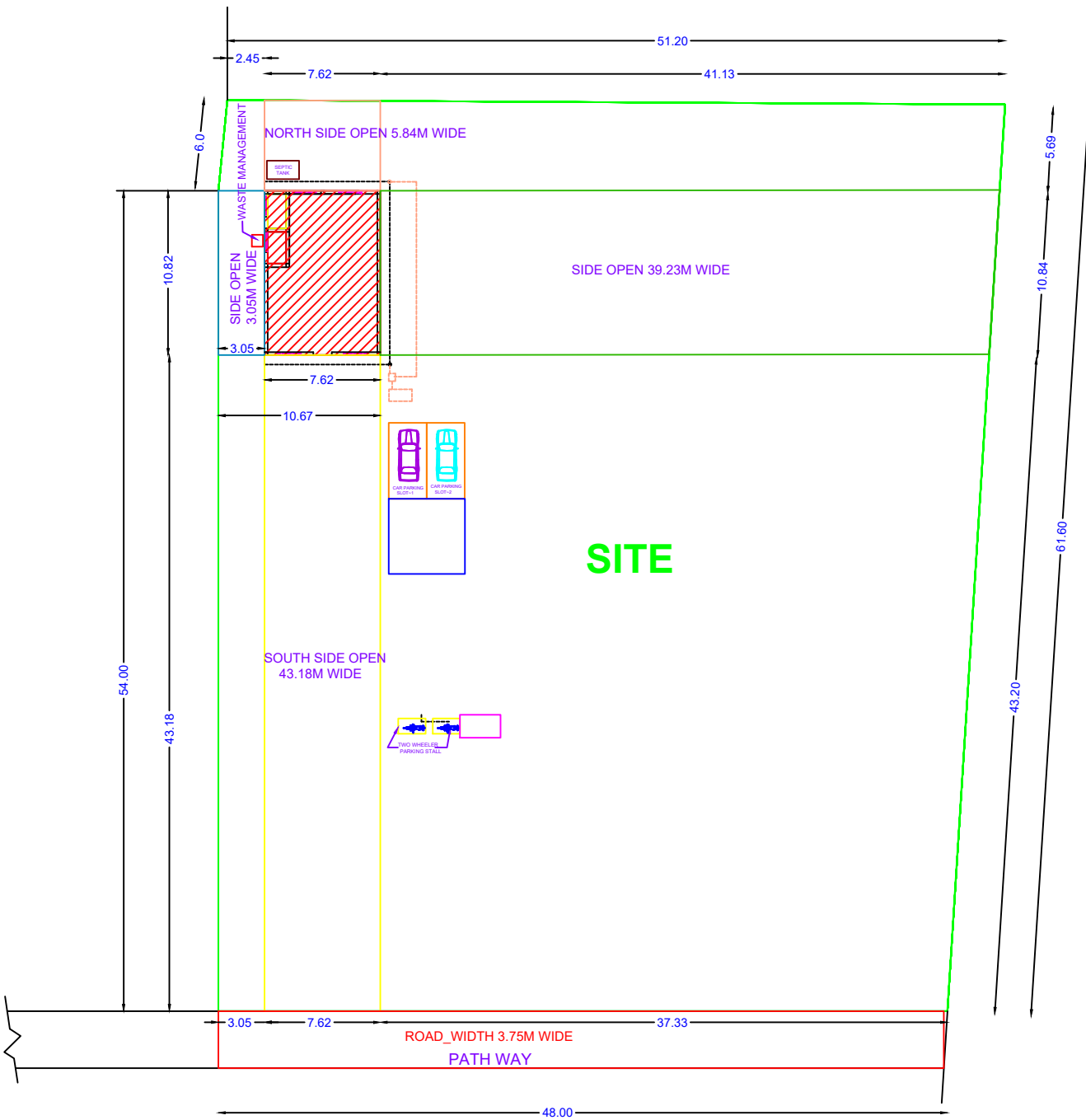
SITE PLAN
