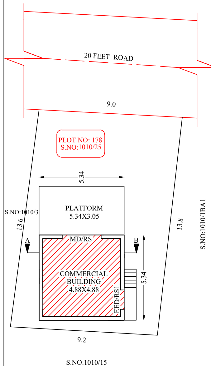
SITE PLAN
