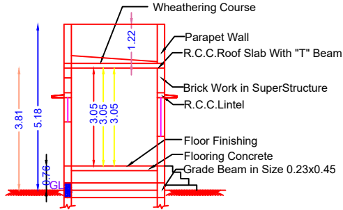
SECTION ON "PQ" SCALE 1:100
