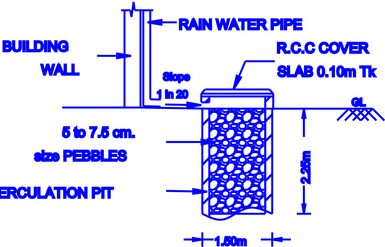
RAIN WATER HARVESTING TRENCH PIT DETAILS
