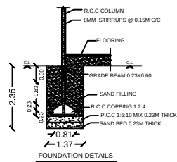
FOUNDATION DETAILS
