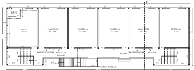
GROUND FLOOR PLAN (Block-01)
