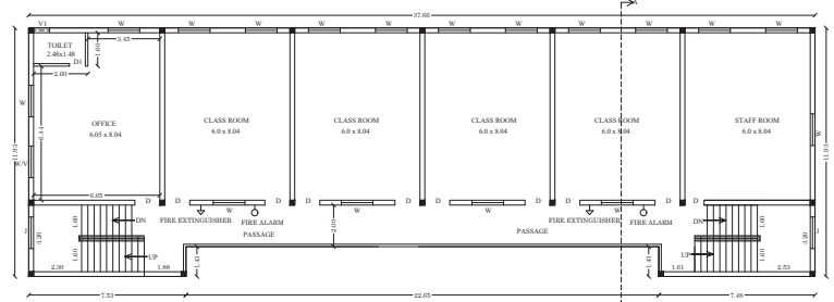
FIRST FLOOR PLAN (Block-01)
