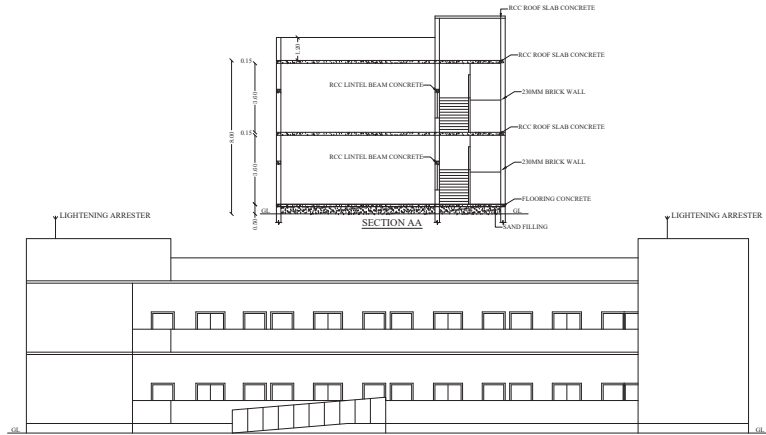
ELEVATION (Block-01)
