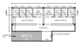
GROUND FLOOR PLAN (Block-02)
