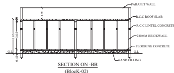
SECTION ON-BB (Block-02)
