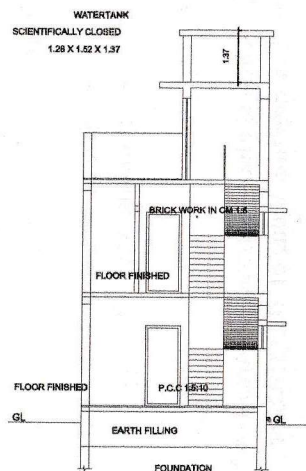
SECTION "A-B"
