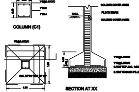
COLUMN DETAILS
