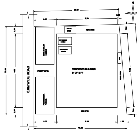
SITE PLAN
