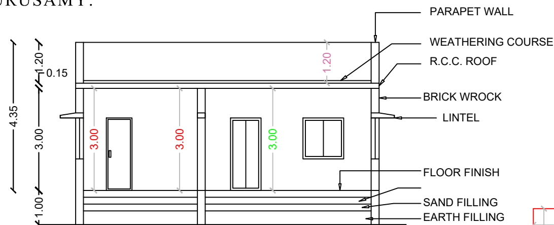
SECTION ON "XX"
