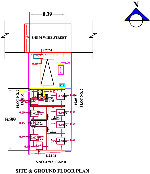
SITE & GROUND FLOOR PLAN
