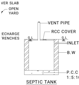
SEPTIC TANK
