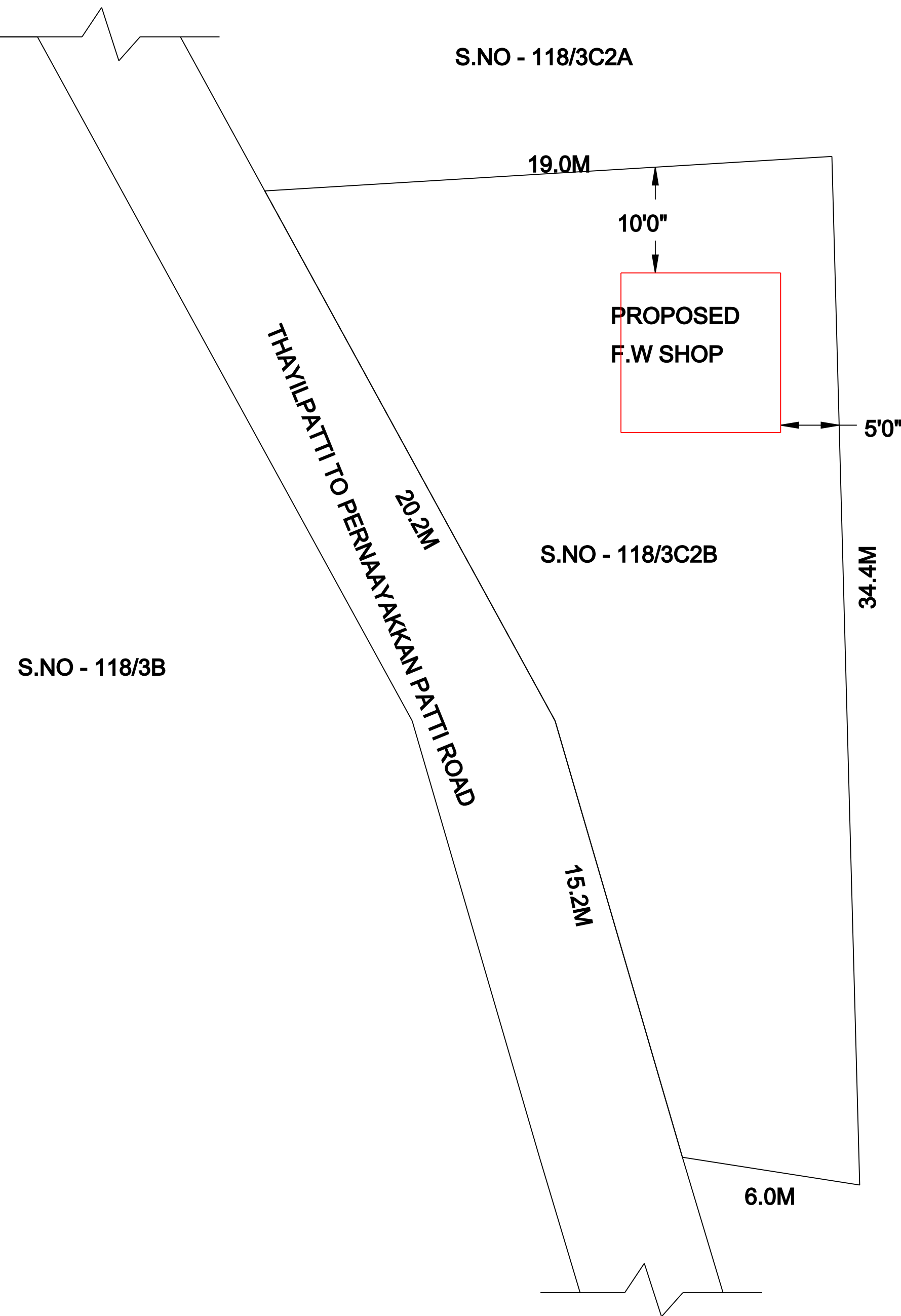
SITE PLAN NOT TO SCALE
