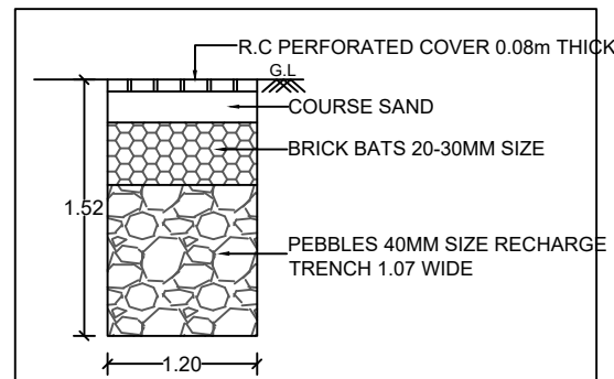
SECTIONAL VIEW OF RAIN WATER HARVESTING TRENCH
