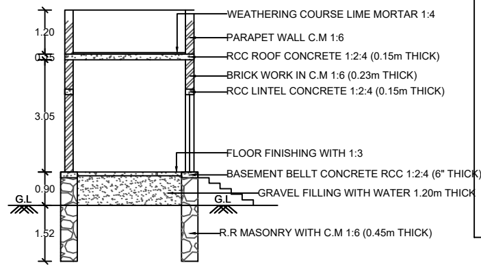
SECTION PLAN
