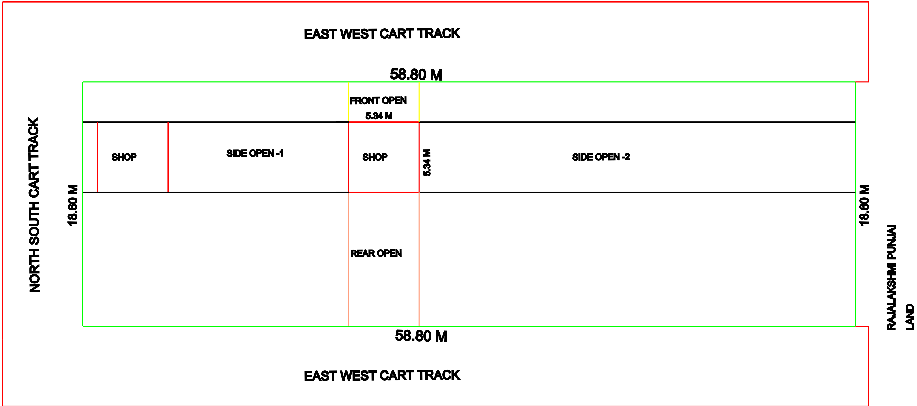
SITE PLAN
