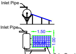
DETAILS OF SOLAR WATER HEATER
