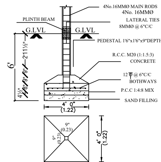
FOUNDATION DETAIL (SCALE: 1:50)
