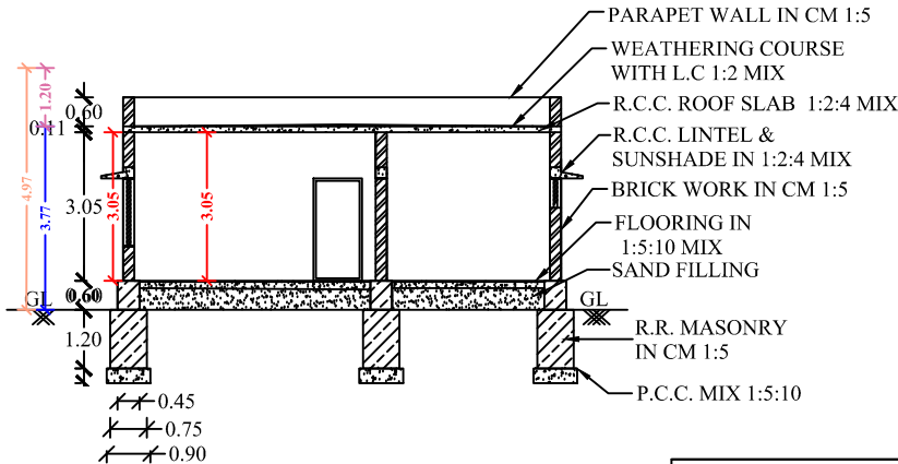
SECTION OF "AB"
