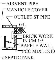
SEPTICTANK
