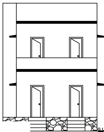
FRONT ELEVATION
