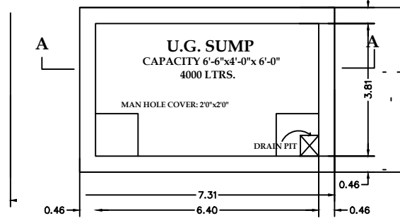
SUMP DETAIL SCALE 1"=4'0"
