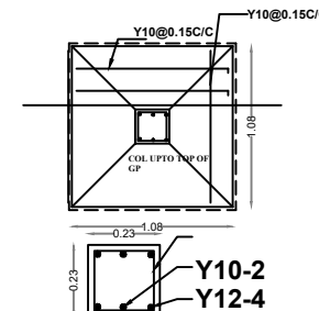
COLUMN (C1)
