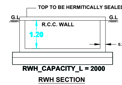
RWH SECTION
