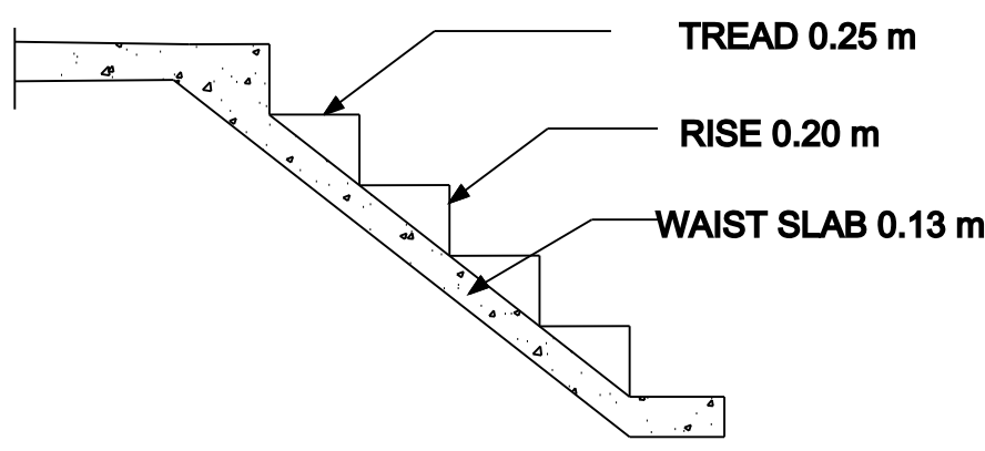
STAIR DETAILS
