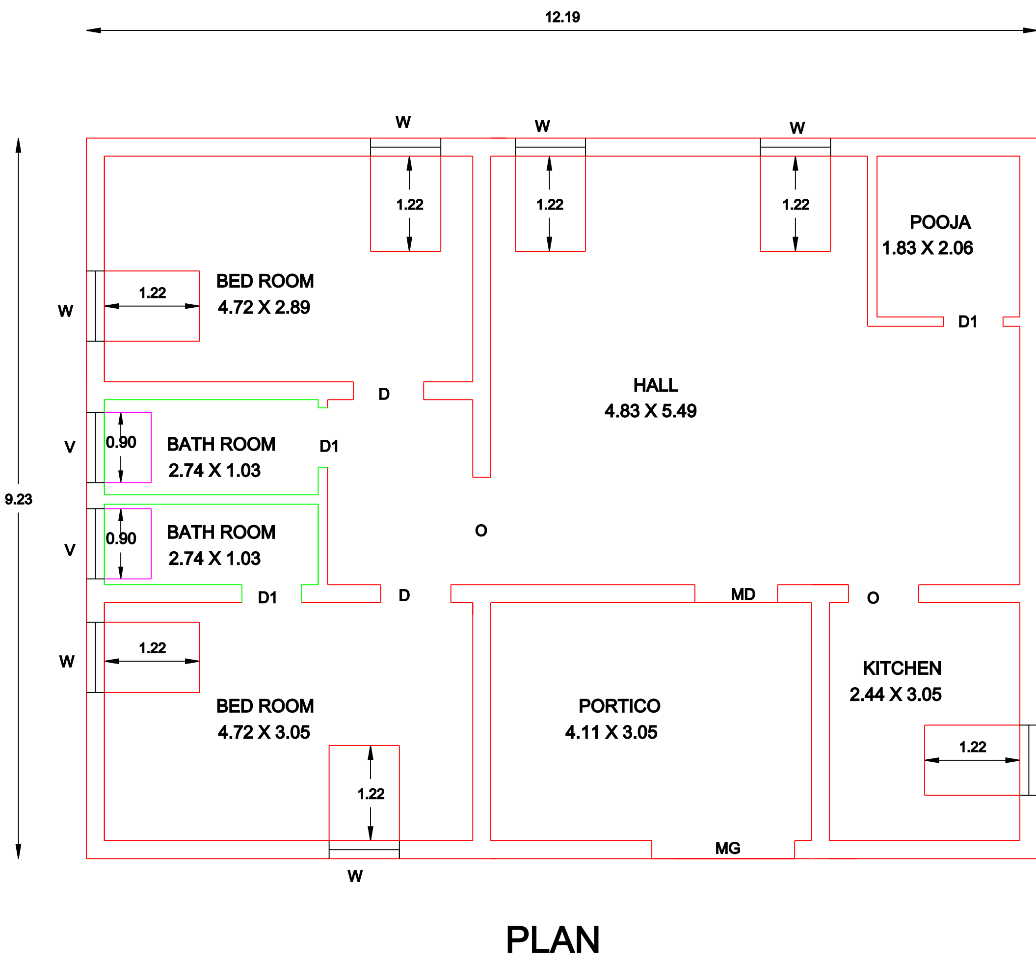
PLAN
