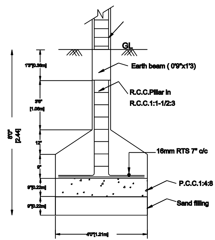
FOUNDATION DETAILS
