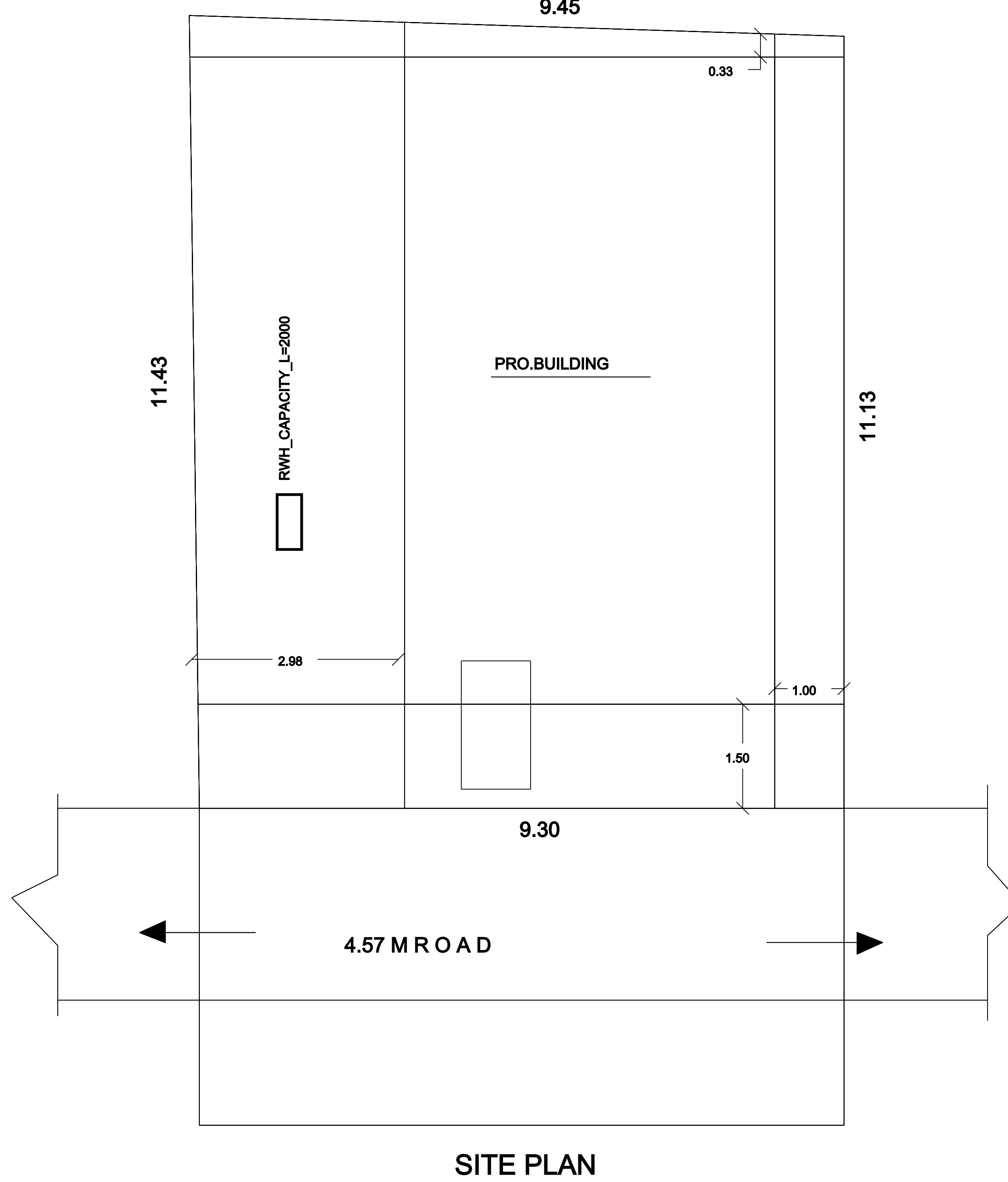
SITE PLAN
