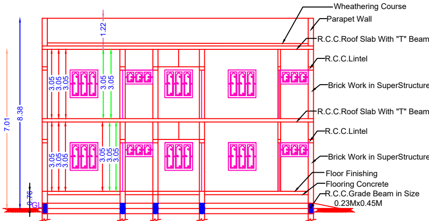
SECTION ON "PQ" SCALE 1:100
