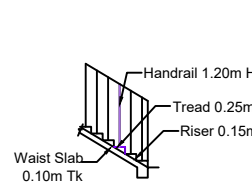
DETAILS OF STAIR CASE (SCALE 1:100)
