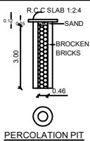
DETAILS OF FILTER BED & WELL
