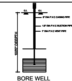
BORE WELL
