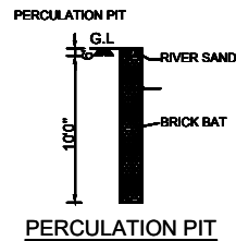
PERCUSSION PIT
