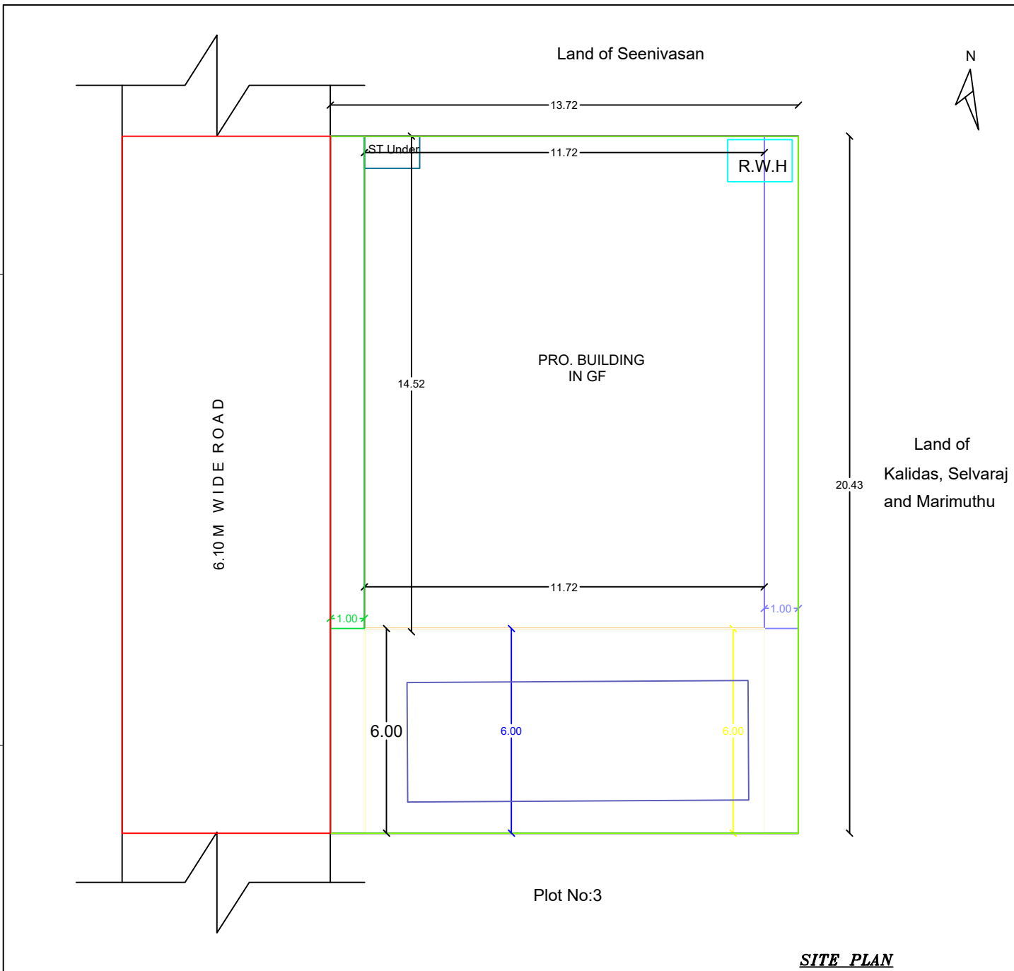
SITE PLAN
