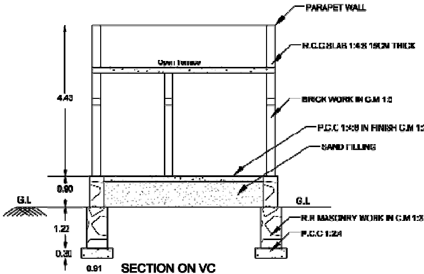
SECTION ON VC
