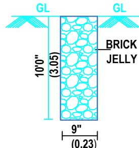
PERCOLATION PIT
