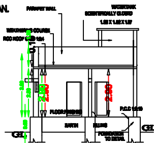
SECTION "A-B"
