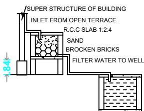
RAINWATER HARVESTING
