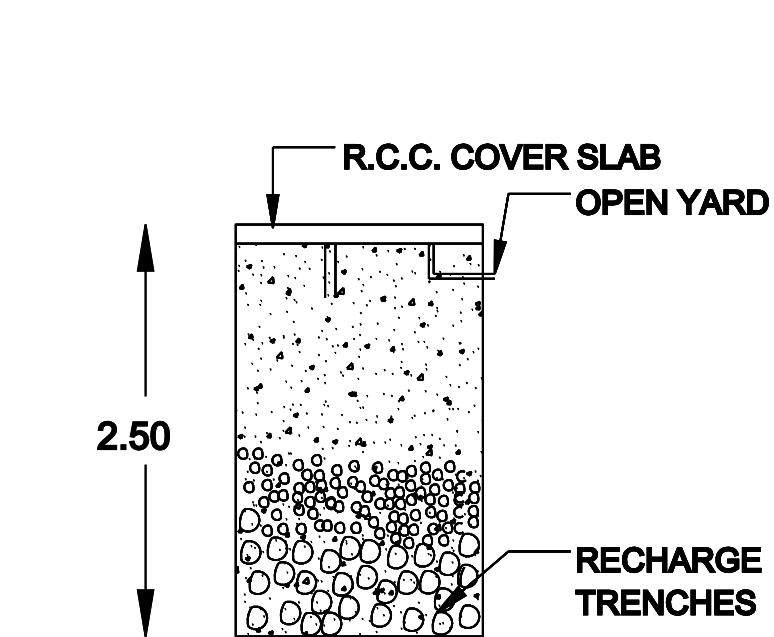
SECTION C-C'
