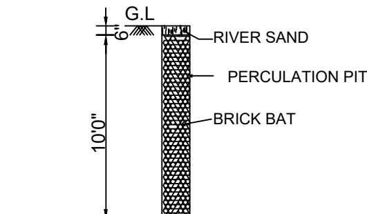
PERCOLATION PIT
