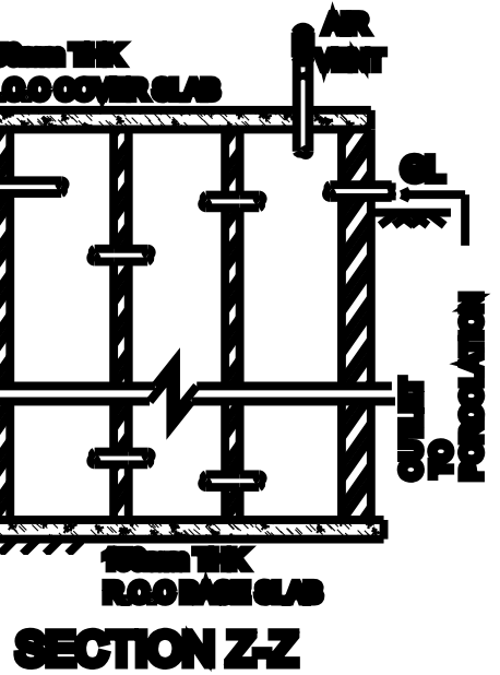
SECTION Z-Z
