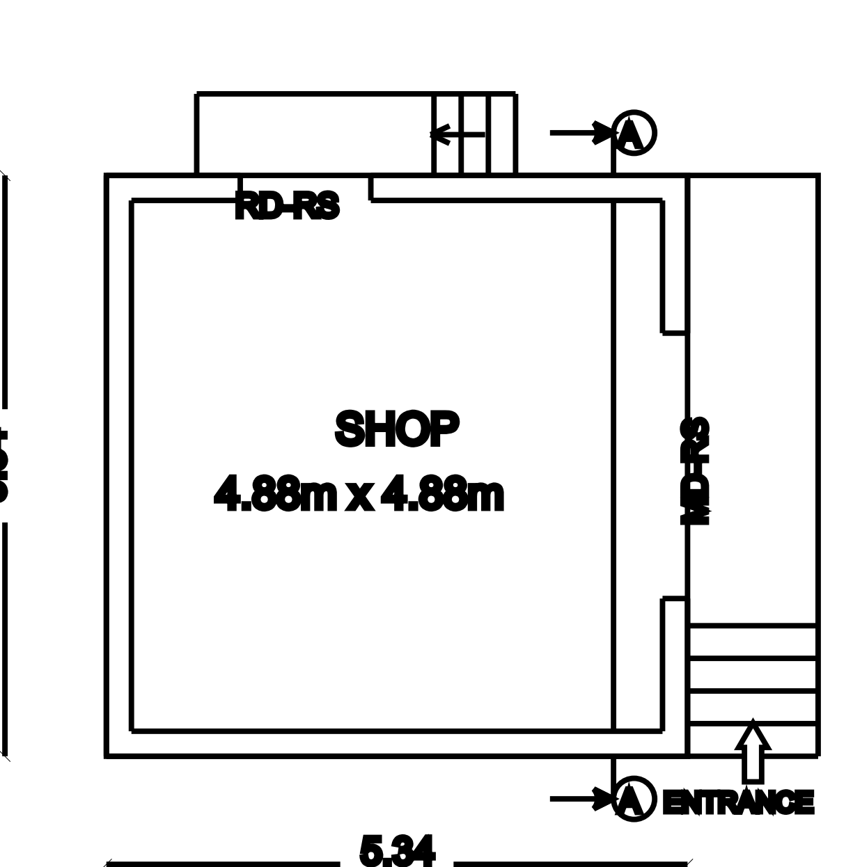
FLOOR PLAN
