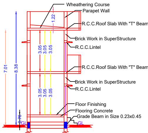
SECTION ON "PQ" SCALE 1:100
