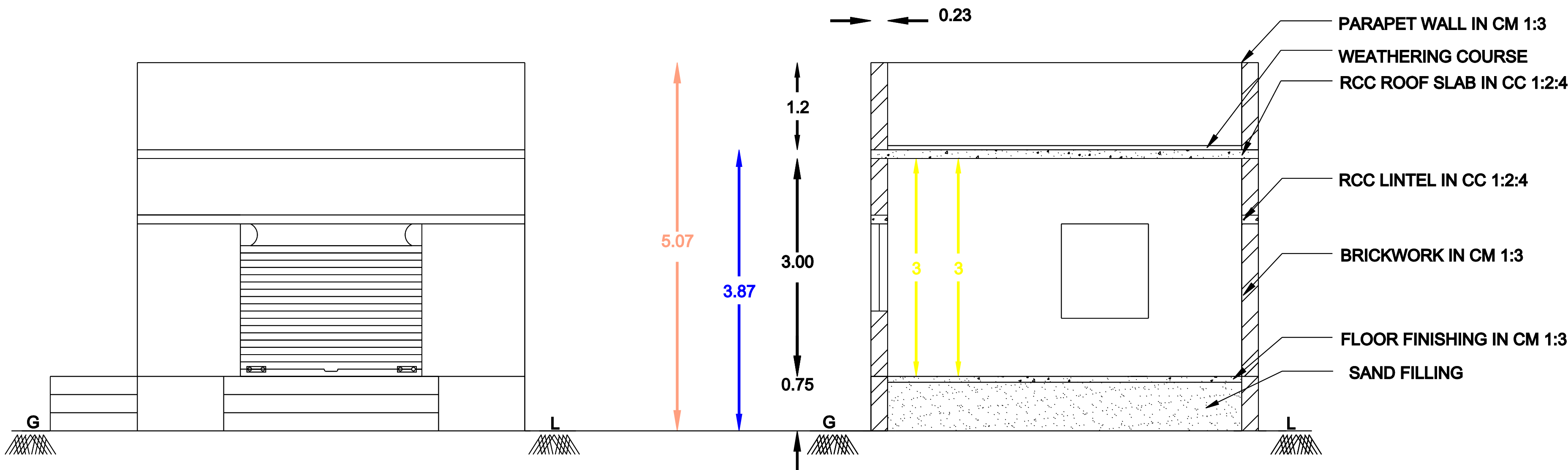
FRONT ELEVATION NORTH SIDE
