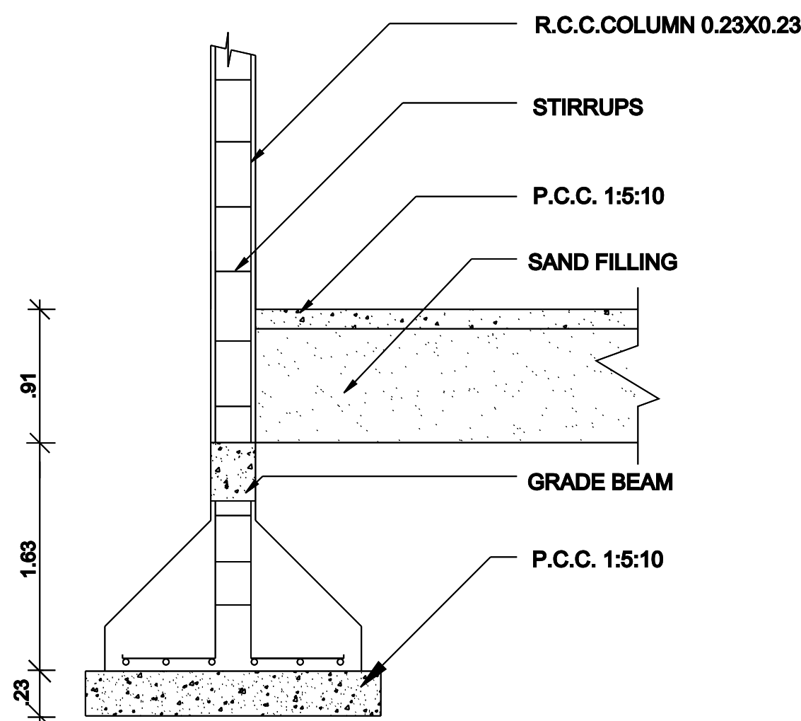
COLUMN DETAIL
