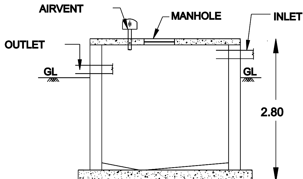
SECTION B-B'
