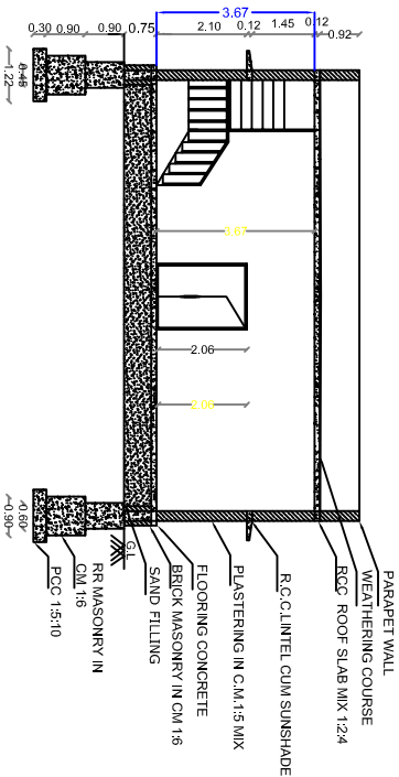
SECTION ON AA
