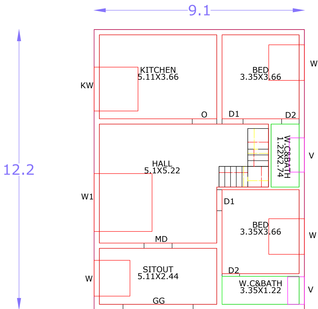
GROUND FLOOR
