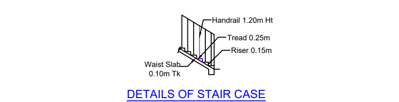
DETAILS OF STAIR CASE
