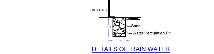
DETAILS OF RAIN WATER PERCOLATION PIT
