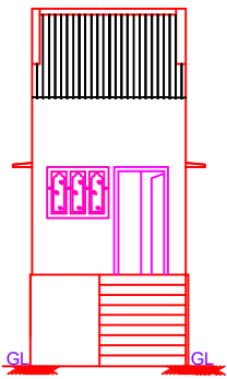
FRONT ELEVATION
