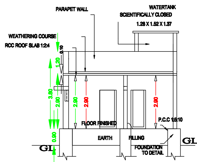
SECTION "A-B"
