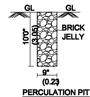
PERCULATION PIT
