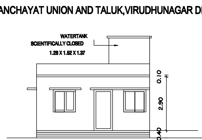
NORTH FRONT ELEVATION.
