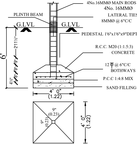
FOUNDATION DETAIL [SCALE: 1:50]
