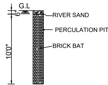
PERCULATION PIT
