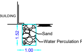
DETAILS OF RAIN WATER PERCOLATION PIT (SCALE 1:100)
