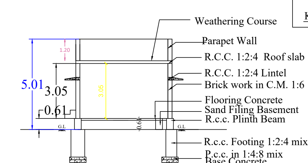
SECTION - "AB"
