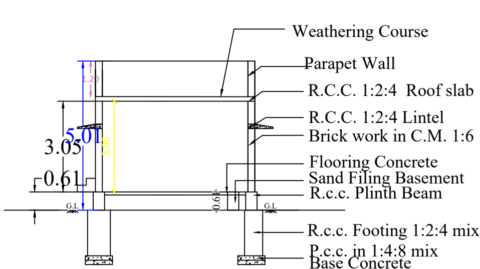
SECTION - "AB"
