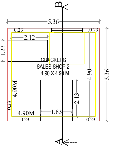
GROUND FLOOR PLAN-2
