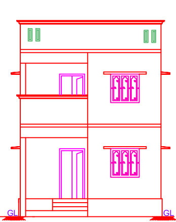
FRONT ELEVATION
