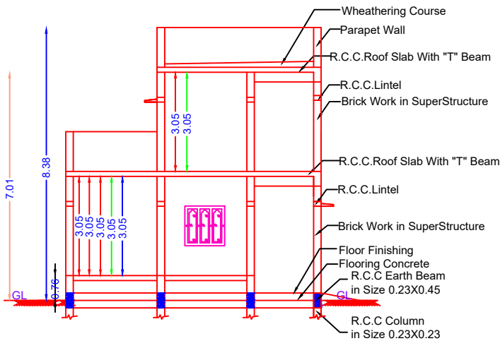
SECTION ON "PQ" (SCALE 1:100)
