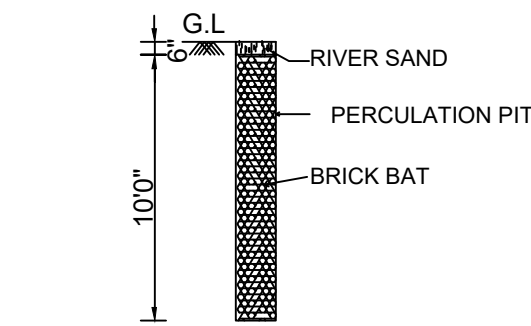
PERCULATION PIT
