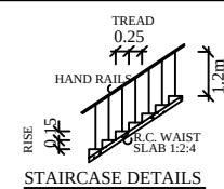
STAIRCASE DETAILS
