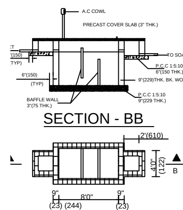
LAN OF SEPTIC TANK
