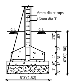
COLUMN FOUNDATION DETAIL
